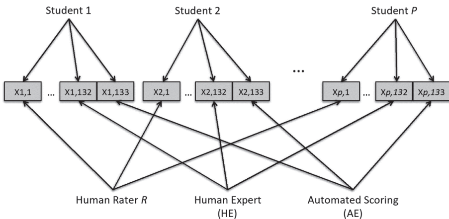
Figure 1: Data Structure
